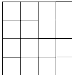
Word-matrix
